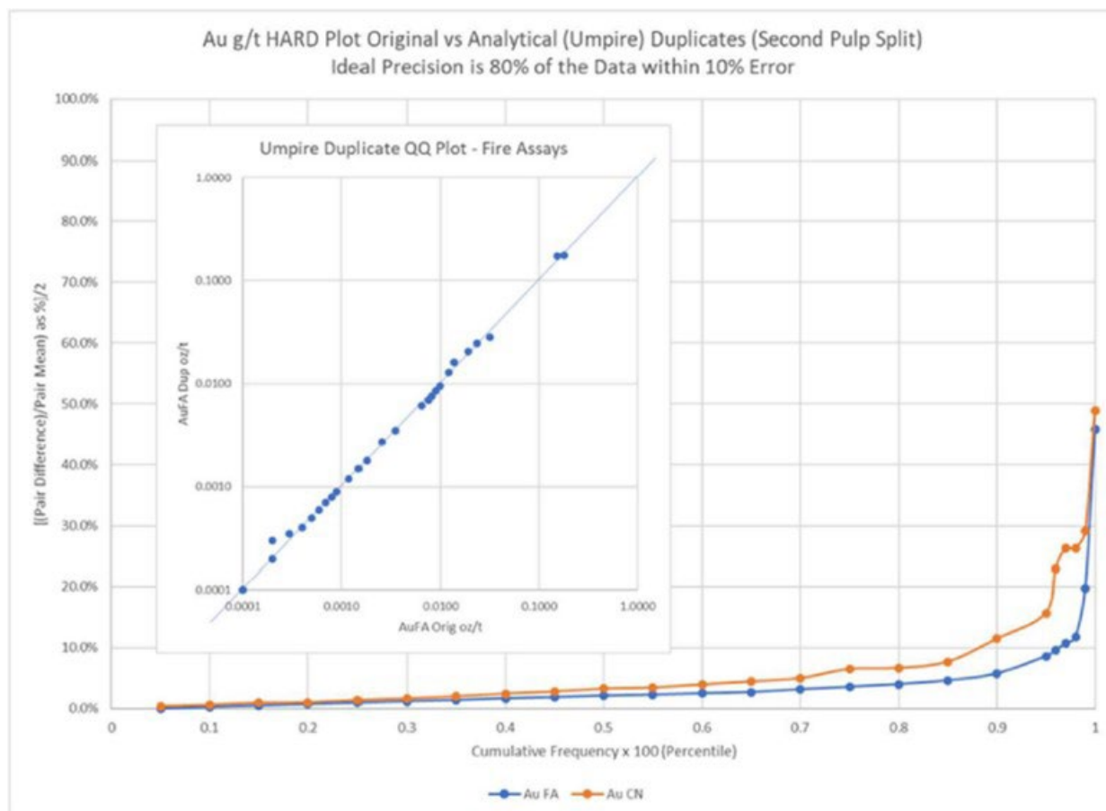
Figure 8-9: Umpire Analytical Duplicate HARD Plot for Fire Assay (AuFA) and Cyanide Soluble (AUCN) Analyses. Inset QQ Plot of Original vs. Umpire Results
