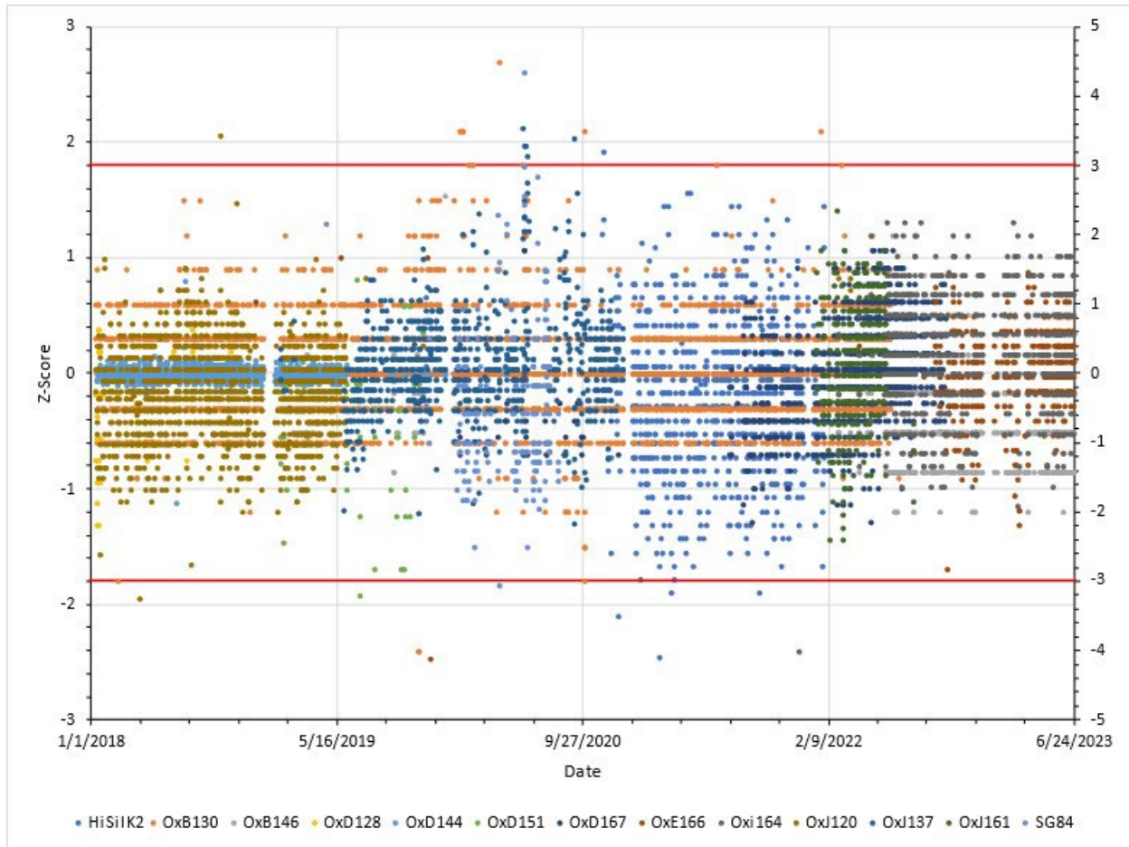
Figure 8-5: Z-Scores of all CRM Results (2018 – June 2023)
